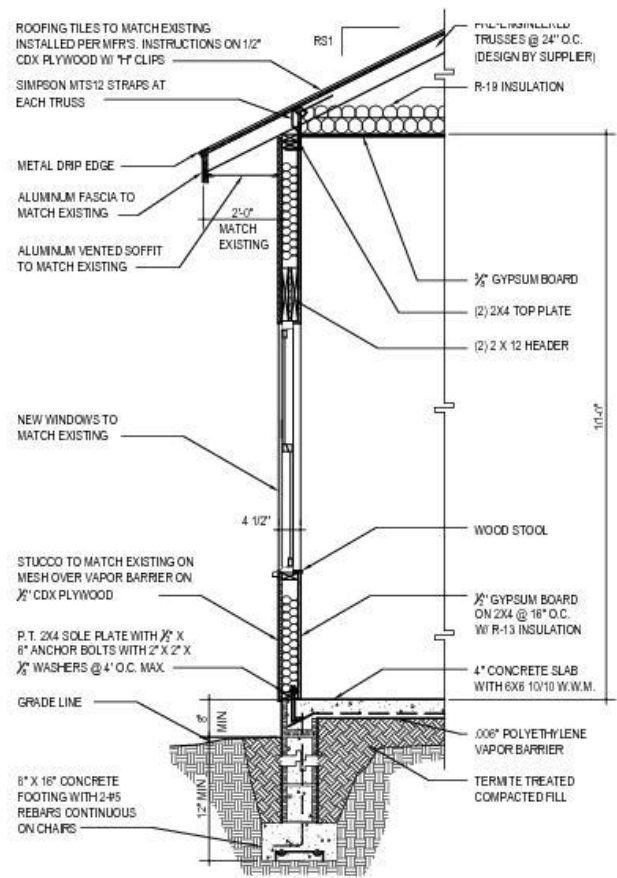
1 TYPICAL WALL SECTION 3/4" = 1'-0" STUD-100
